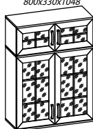
22.1.ШВ 105.80.2 800x330x1048
